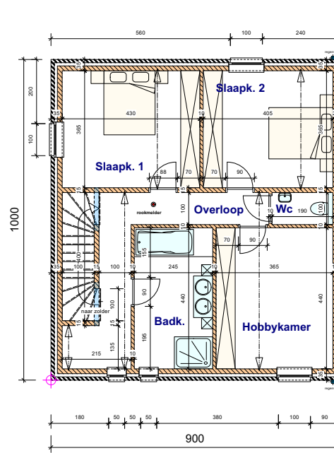
Verdieping LOT 78
